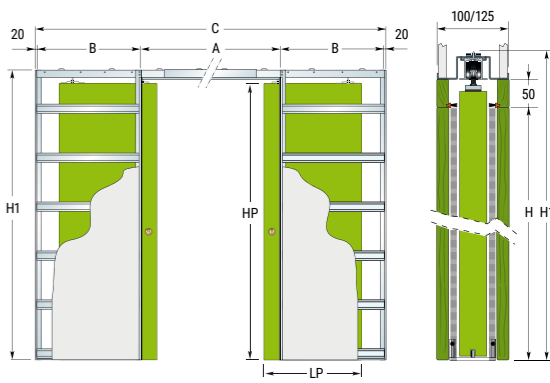
DOUBLE POCKET DIMENSION TABLE DOUBLE POCKET DIMENSION TABLE
