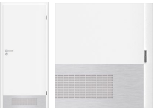
STEEL KICK-PLATE WITH VENTILATION GRILLE STEEL KICK-PLATE WITH VENTILATION GRILLE two-sided two-sided
