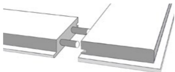
FRAME CONSTRUCTION FRAME CONSTRUCTION construction elements connected with mounting pins construction elements connected with mounting pins
