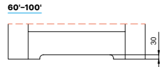
HEIGHT OF VENTILATION UNDERCUT IN FRAME DOORS, FOR WIDTH 60'-100' 2
