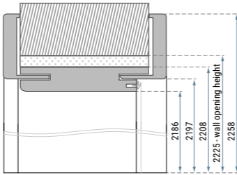
Dimensions of door frame for PN22 door. Dimensions of door frame for PN22 door.
