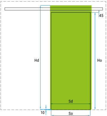
AERO SYSTEM DIMENSION TABLE AERO SYSTEM DIMENSION TABLE
