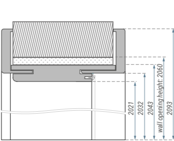
ADJUSTABLE NON-REBATED DOOR FRAME ADJUSTABLE NON-REBATED DOOR FRAME
