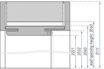
ADJUSTABLE 80 NON-REBATED DOOR FRAME ADJUSTABLE 80 NON-REBATED DOOR FRAME
