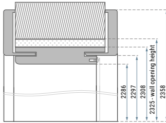
Dimensions of door frame for PN23 door. Dimensions of door frame for PN23 door.
