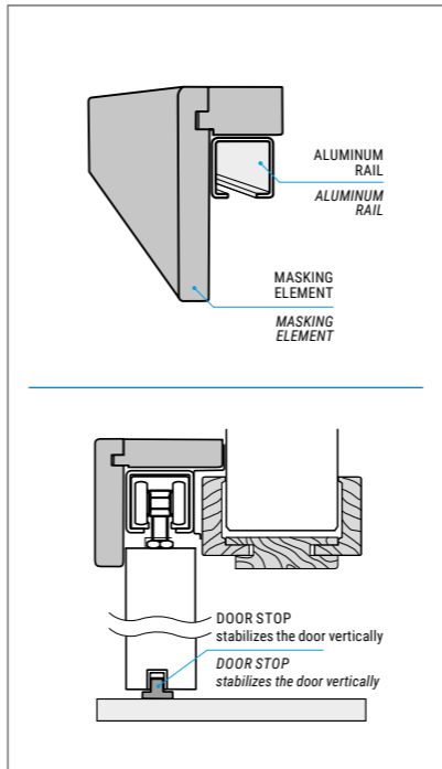
VERTICAL CROSS-SECTION OF THE SLIDING SYSTEM VERTICAL CROSS-SECTION OF THE SLIDING SYSTEM
